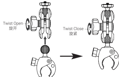
Assemble Claw Mount 组装万向车把支架夹
